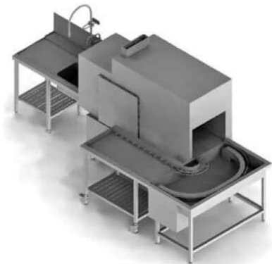
STR 155 Energy/STR 208 Energysingle-tank rack conveyor dishwasher with drying zone
